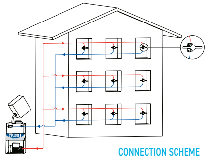
CONNECTION SCHEME
